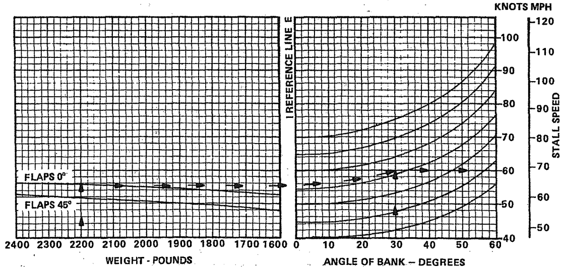
Figure 5-5. Stall Speeds
