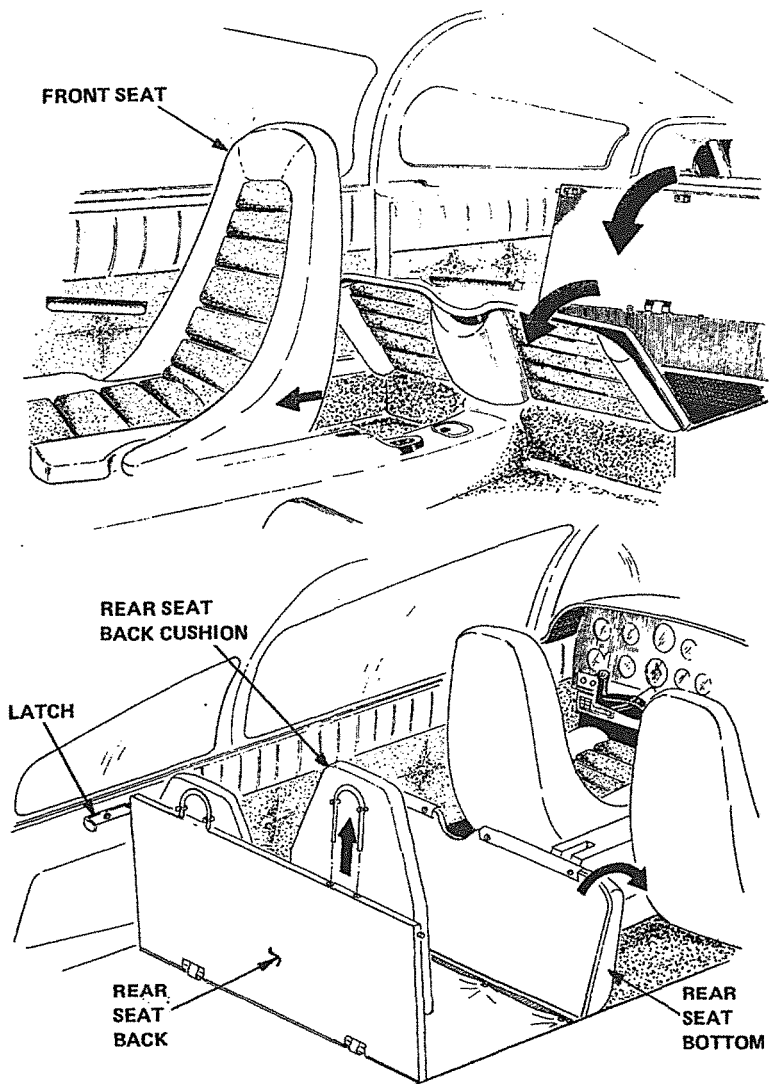
Figure 6-6. Rear Seat Stowage
