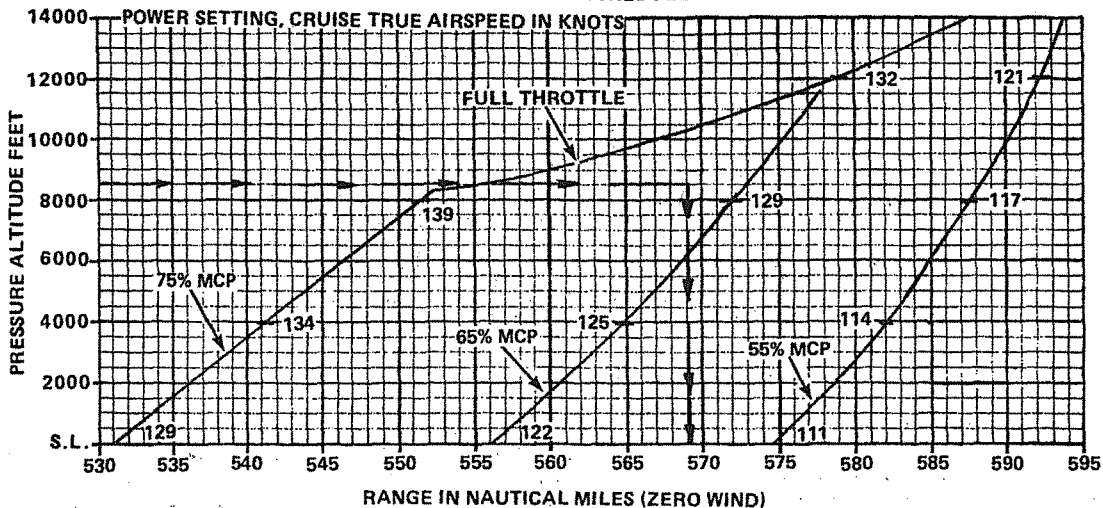
Figure 5-13. Range Profile - 51 Gallons Fuel
