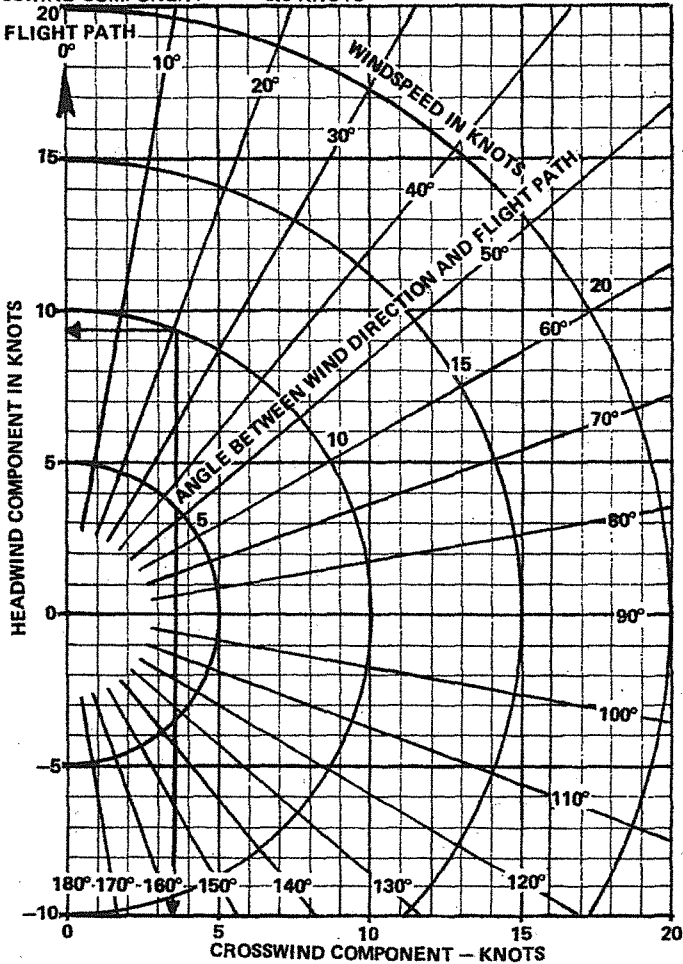
Figure 5-6. Crosswind Component Chart
