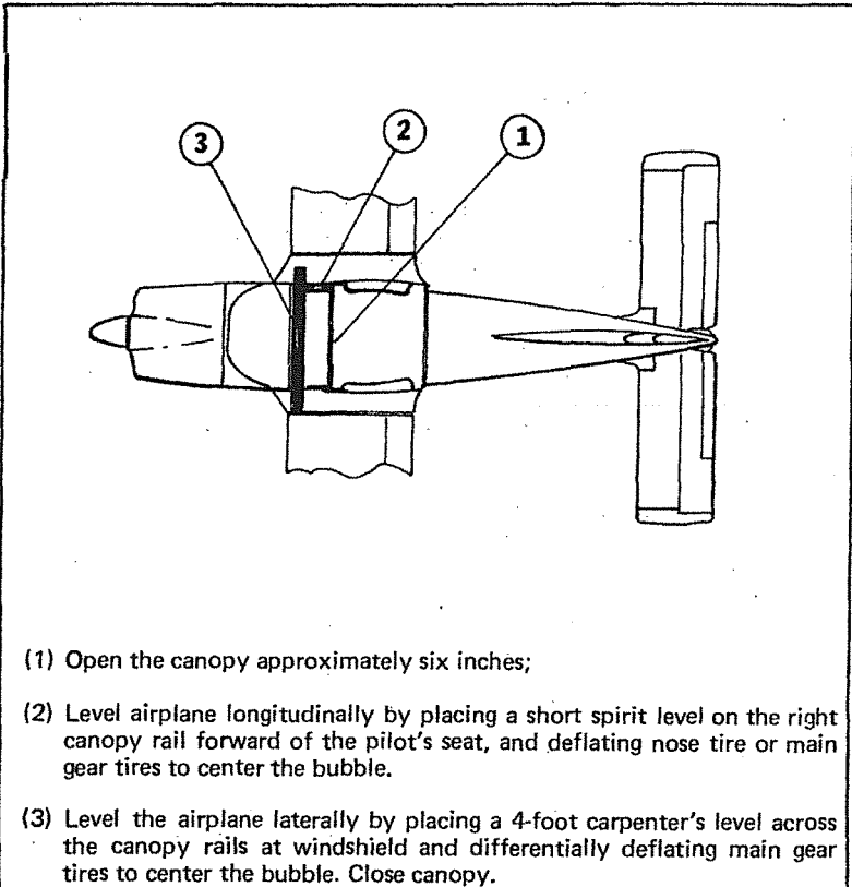
Figure 6-1. Airplane Leveling
