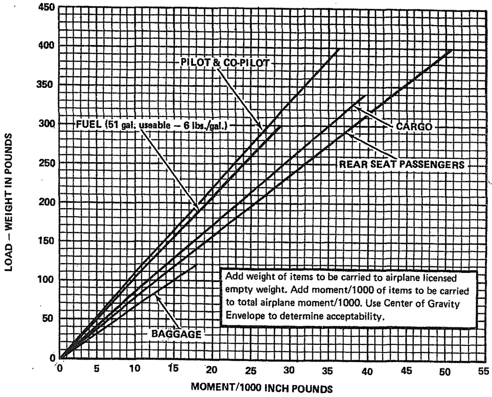
Figure 6-4. Loading Graph
