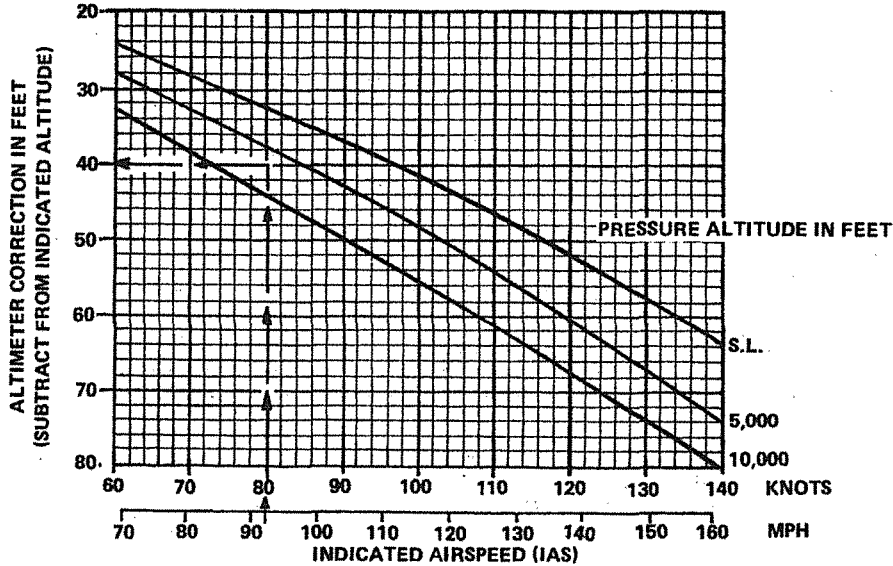
Figure 5-4. Altimeter Correction – Alternate System
