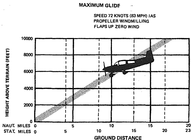
Figure 3.1 Maximum Glide
