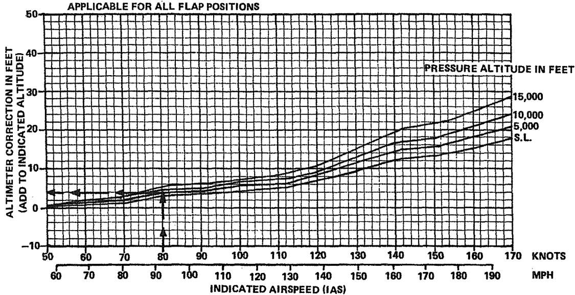
Figure 5-3. Altimeter Correction – Normal System
