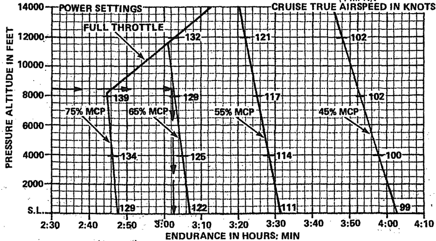
Figure 5-14. Endurance Profile — 37 Gallons Fuel
