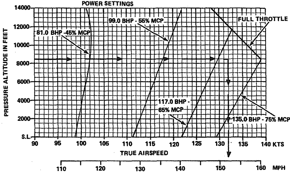
Figure 5-11. Cruise Speeds
