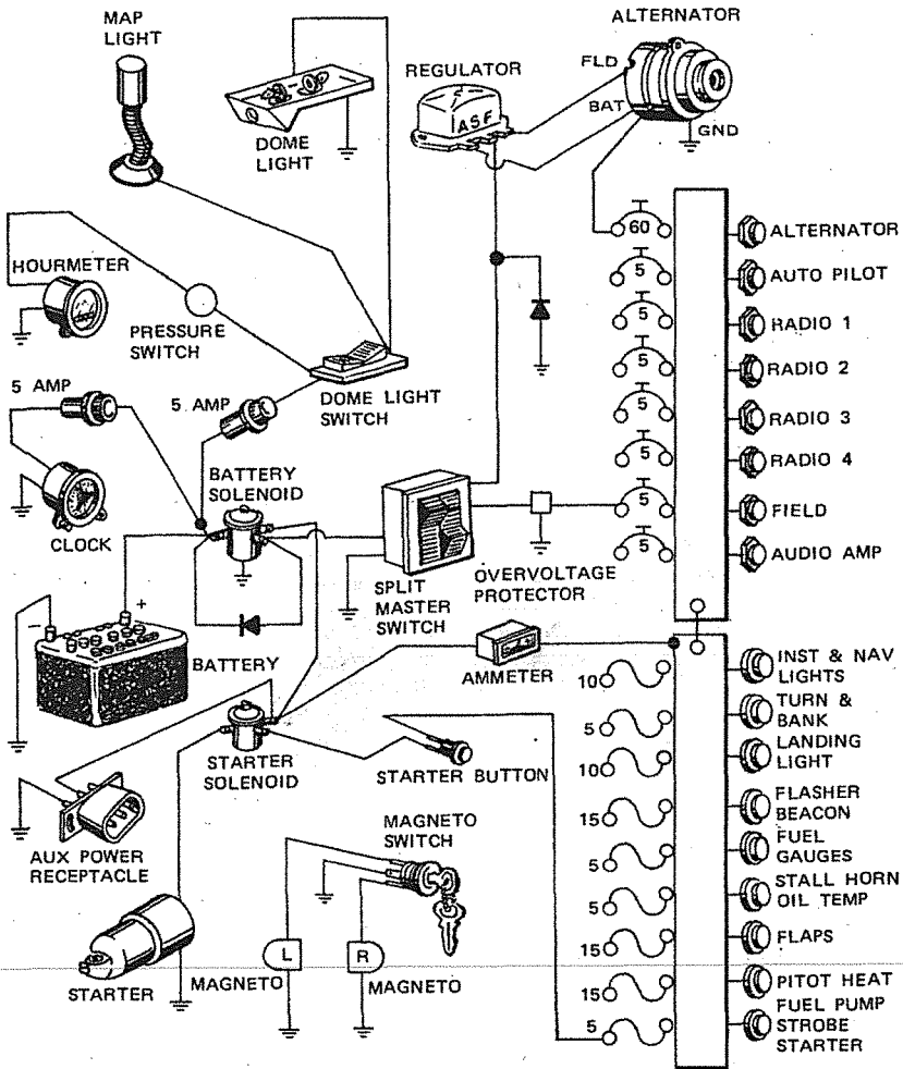
Figure 7-3, Electrical System
