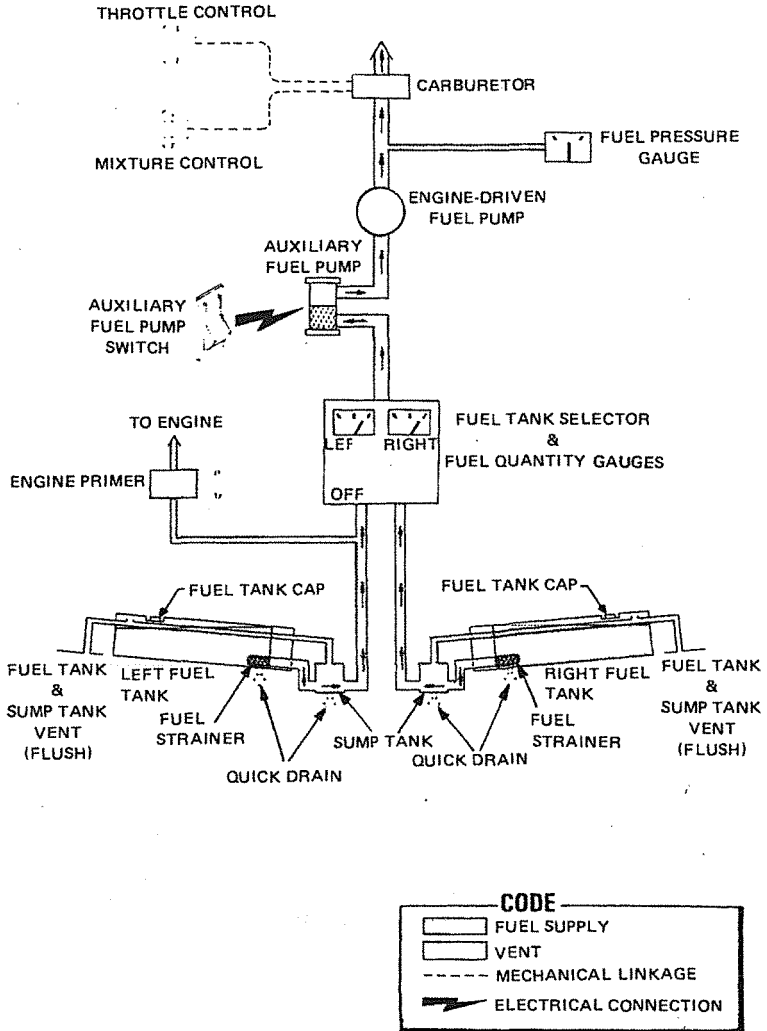
Figure 7-2 Fuel System
