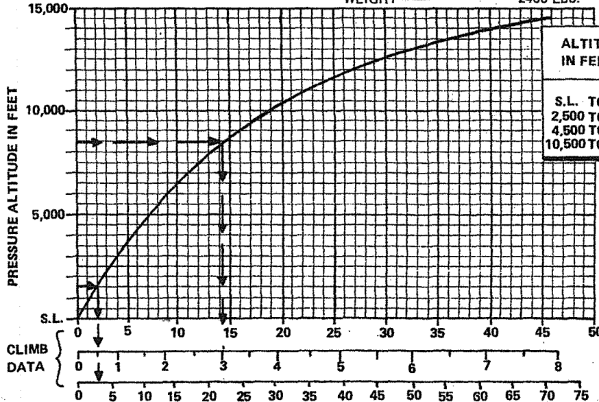
Figure 5-9. Time Fuel and Distance to Climb
