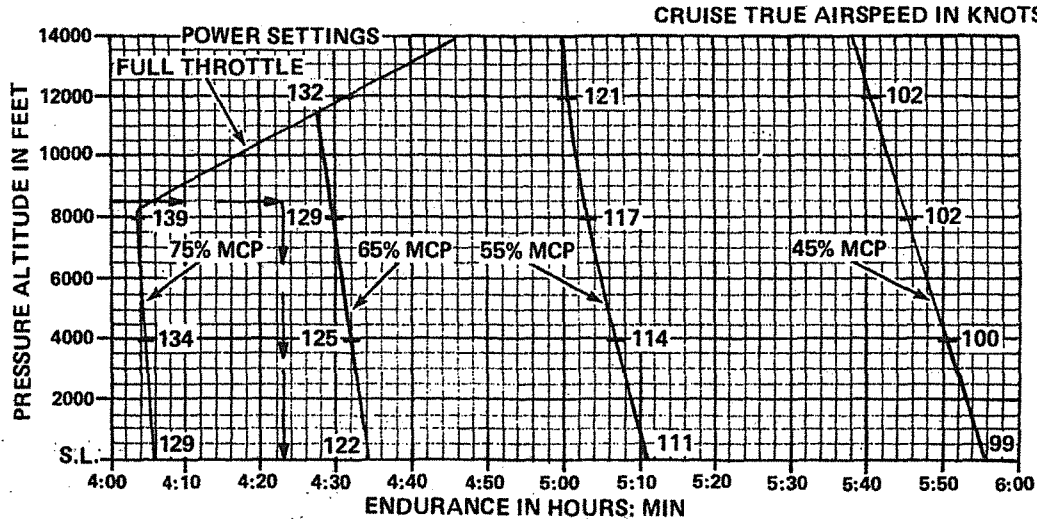
Figure 5-15. Endurance Profile - 51 Gallons Fuel
