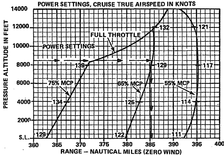
Figure 5-12. Range Profile-37 Gallons Fuel
